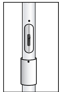
Internal halyard base detail
