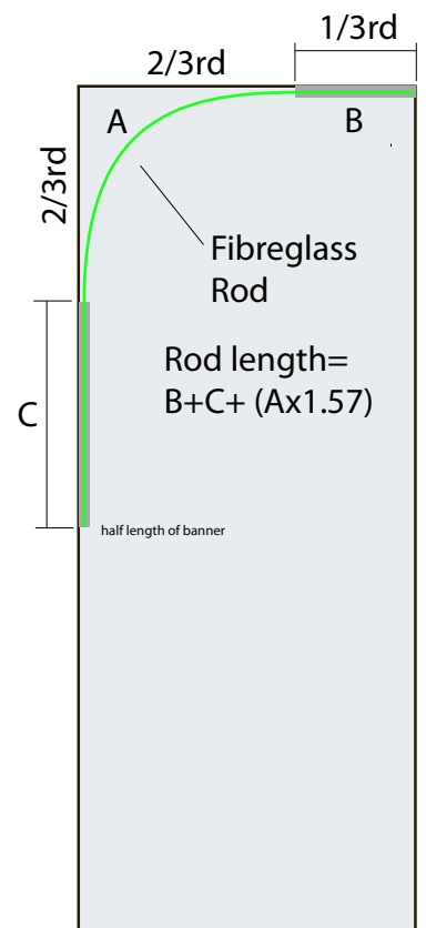
Banner and Fibreglass Rod Batten Arrangement
