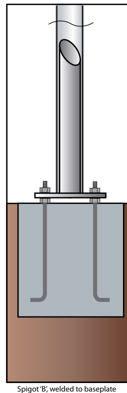
Spigot 'B', welded to baseplate
