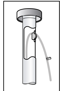
Internal halyard top detail
